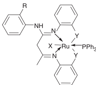
Scheme 6. Proposed structure for the new mononuclear ruthenium(III) complexes.
